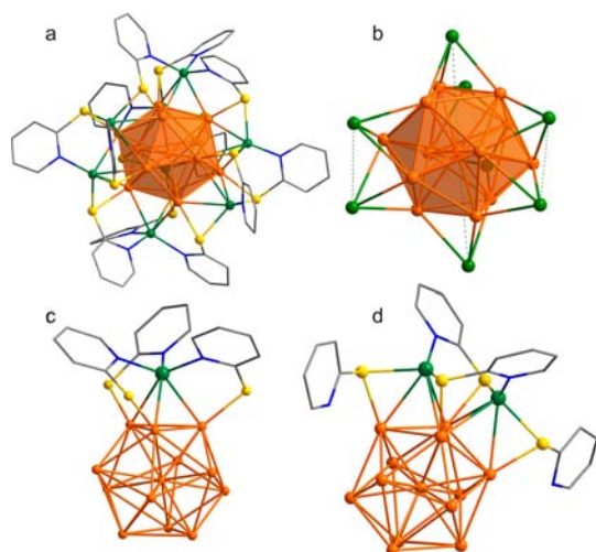
Figure 3. Crystal structure of [\text{Au}_{13}\text{Cu}_8(\text{PPh}_2\text{Py})_{12}]^+ . (a) Overall structure; (b) Distribution of eight Cu atoms on \text{Au}_{13} ; (c,d) Local coordination structures of two types of Cu atoms in [\text{Au}_{13}\text{Cu}_8(\text{PPh}_2\text{Py})_{12}]^+ . Color legend: gold sphere, Au; green sphere, Cu; yellow sphere, S; gray stick, C; blue stick, N. All H atoms are omitted for clarity.
